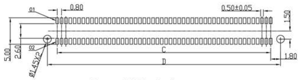
Recommended PC board pattern (TOP VIEW)
